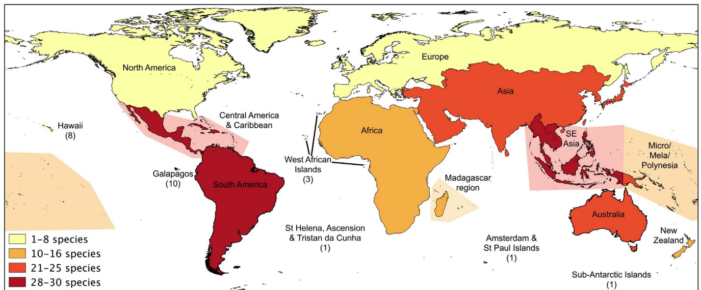
Fig. 2. Regional concentrations of threatened species negatively impacted by domestic dogs Canis familiaris . Number of species is given in parentheses for some small island regions. Also see Table A2 in Appendix A.
